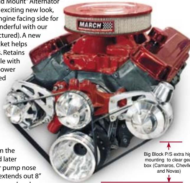
Shown with optional Billet P/S Pump Case
